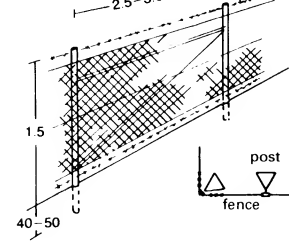
㉒ Wire netting: the bottom either has a small gap (with barbed wire) or is buried
